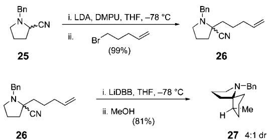
Scheme 2. Carbolithiation of Pyrrolidine 26
