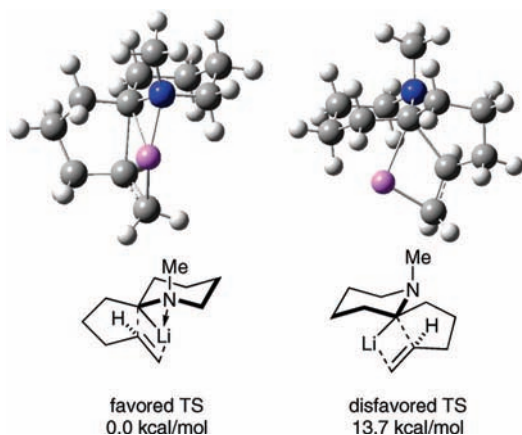
Figure 1. B3LYP/6-31G(d) transition states for the carbolithiation–cyclization of an N -methyl 2-lithiopiperidine.
