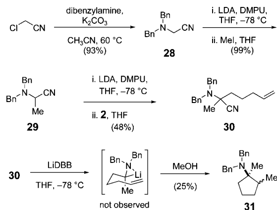
Scheme 3. Sequential Cyanomethylation and Alkylation to Prepare Carbolithiation Precursor 30
