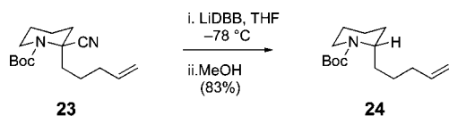
Scheme 1. Reductive Lithation of Boc Aminonitrile 23 Does Not Lead to Cyclization
